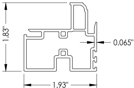
6 KEEPER RAIL
