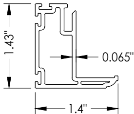
3 SASH STILE
