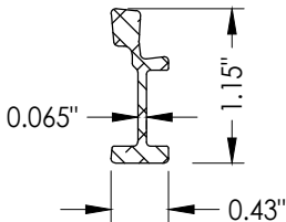
11 SASH REINFORCEMENT
