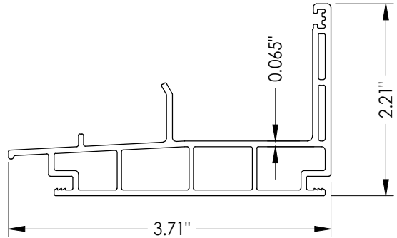
2 SILL
