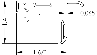
5 LOCK RAIL
